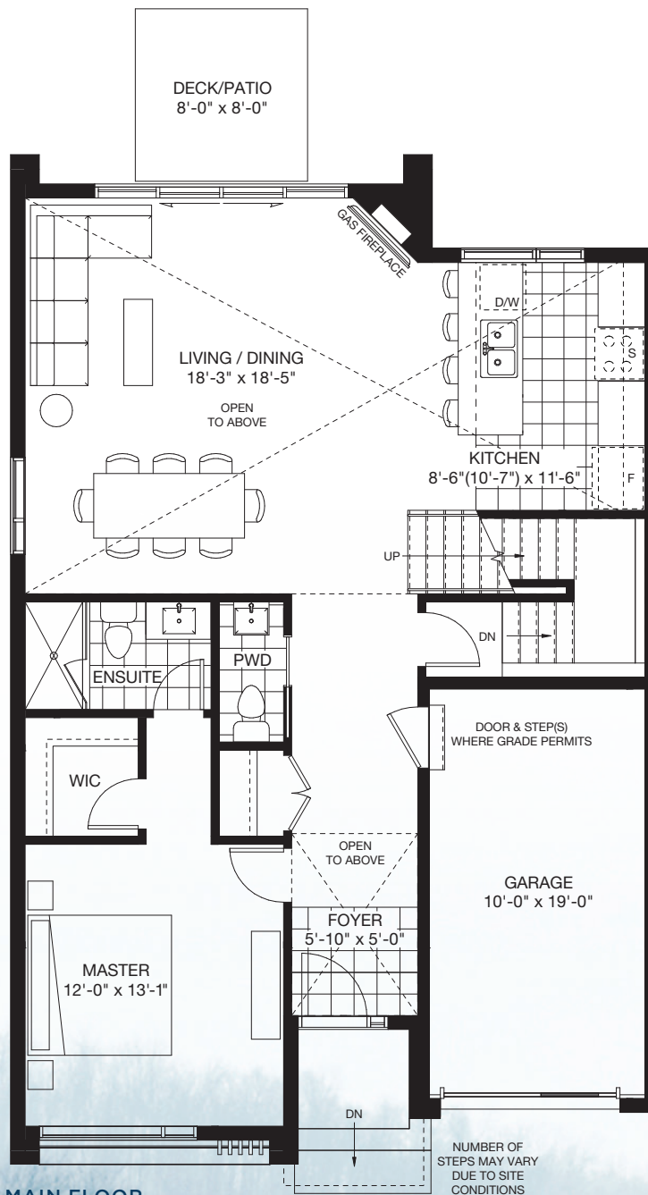
MAIN FLOOR
